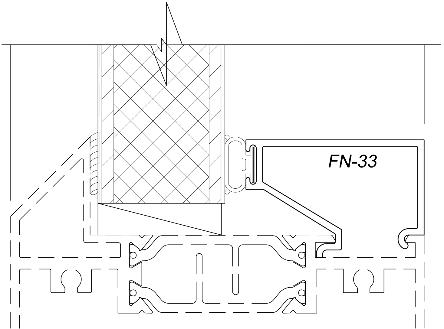
1" Glazing Bead Panel FN-33
