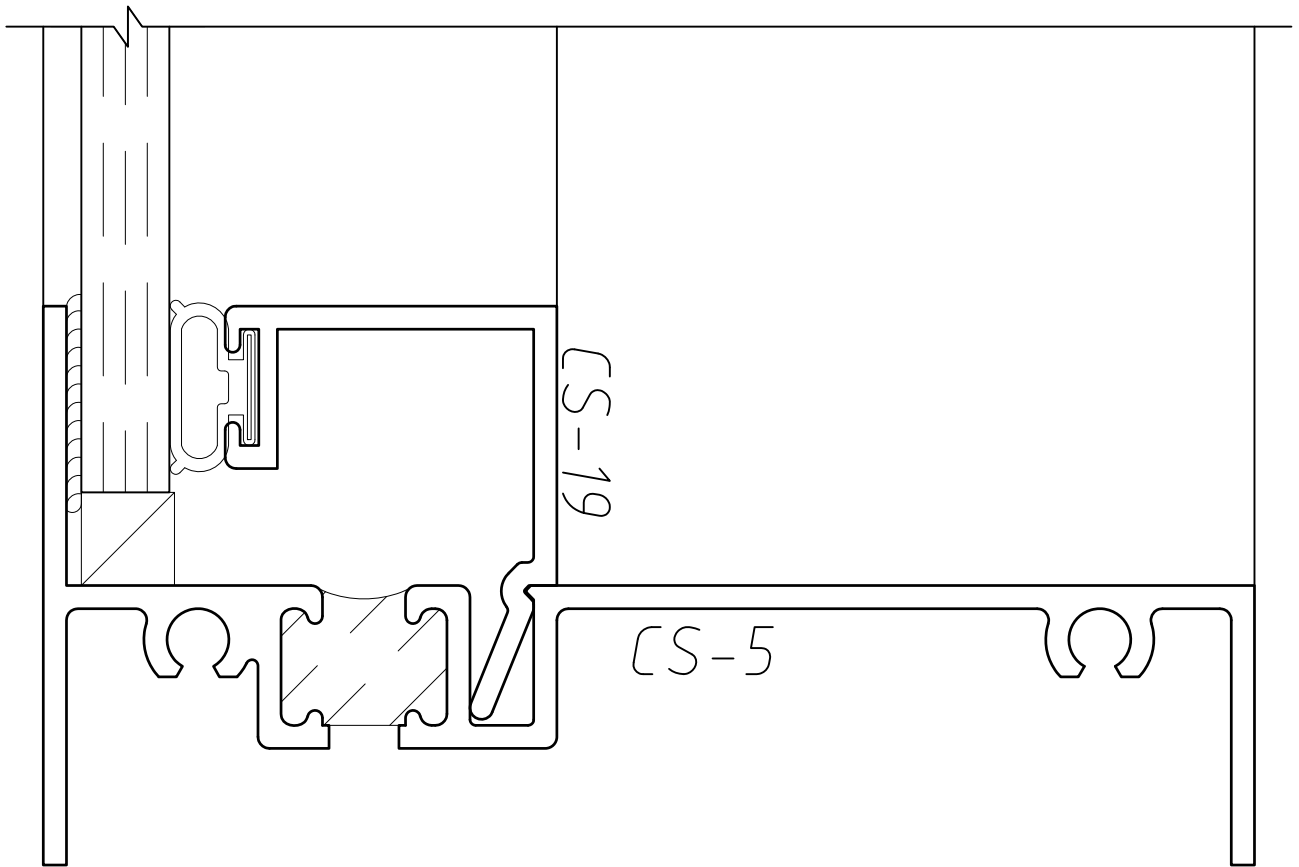
1/4" Glazing Bead CS-19
