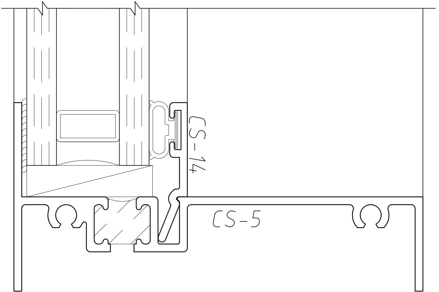
1" Glazing Bead CS-14
