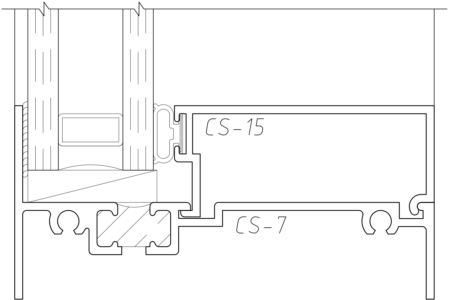
1" Glazing Bead CS-15
