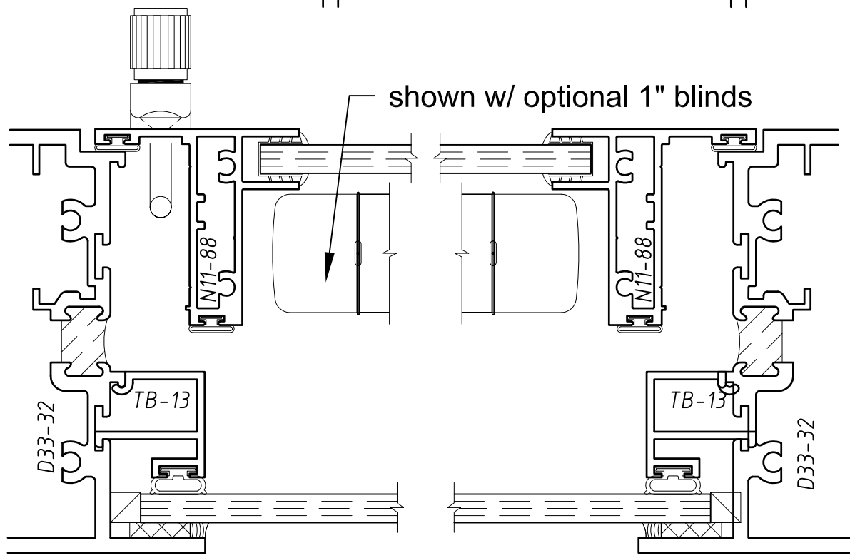
Dual Glazed w/ Take Out Sash
