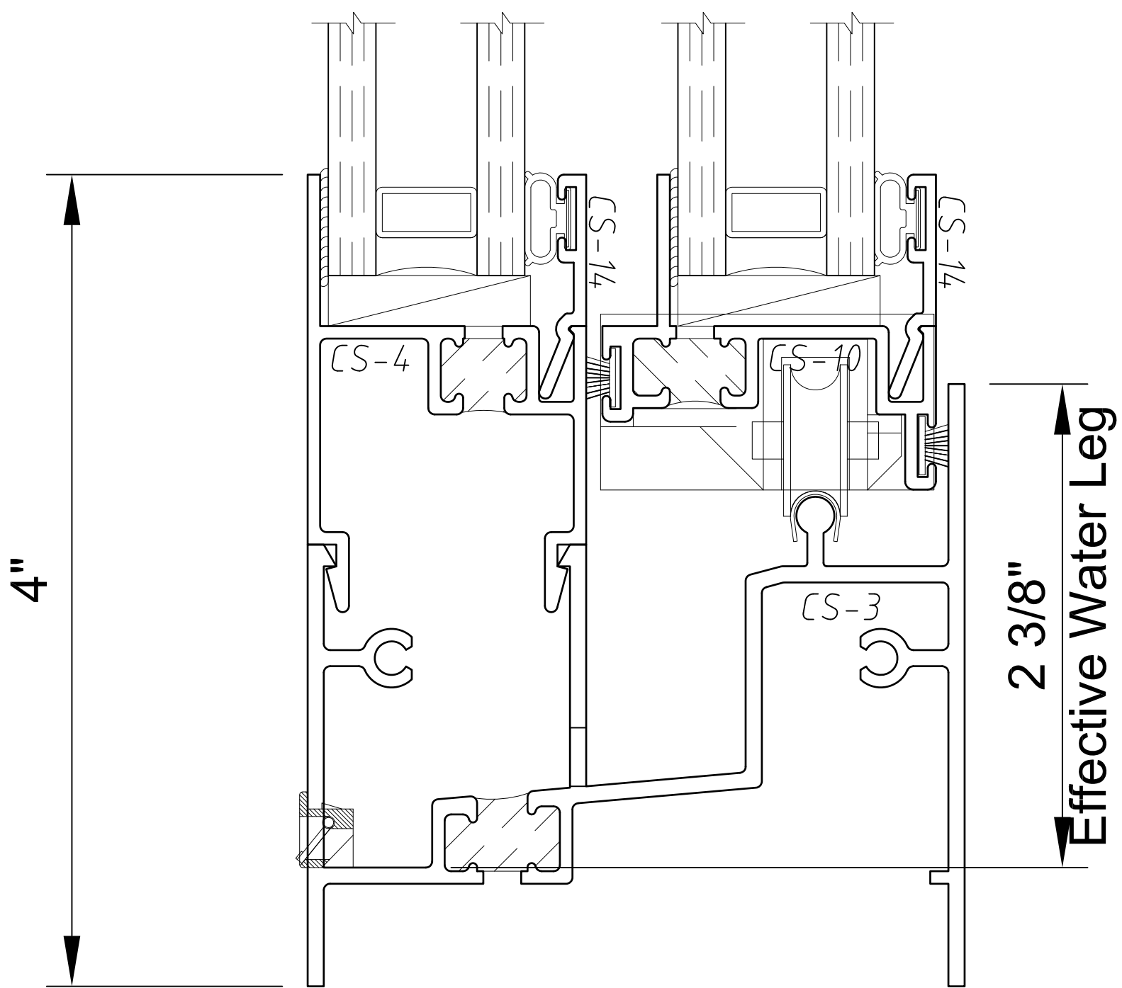
Standard Sill Configuration 10 lbs Water Resistance
