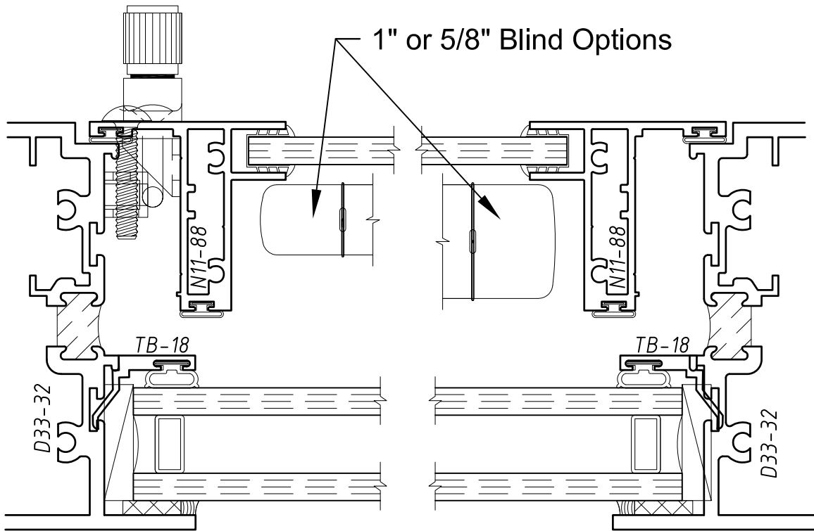
Triple Glazed w/ Hinged Sash
