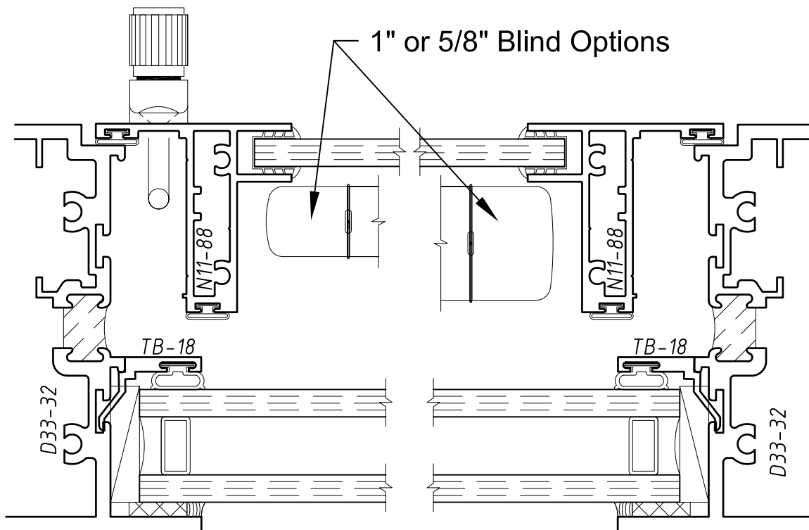
Triple Glazed w/ Take Out Sash
